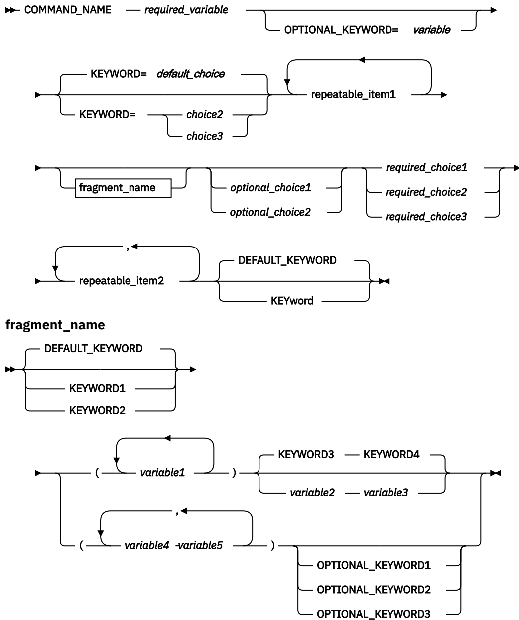
Figure 1. Sample syntax diagram
